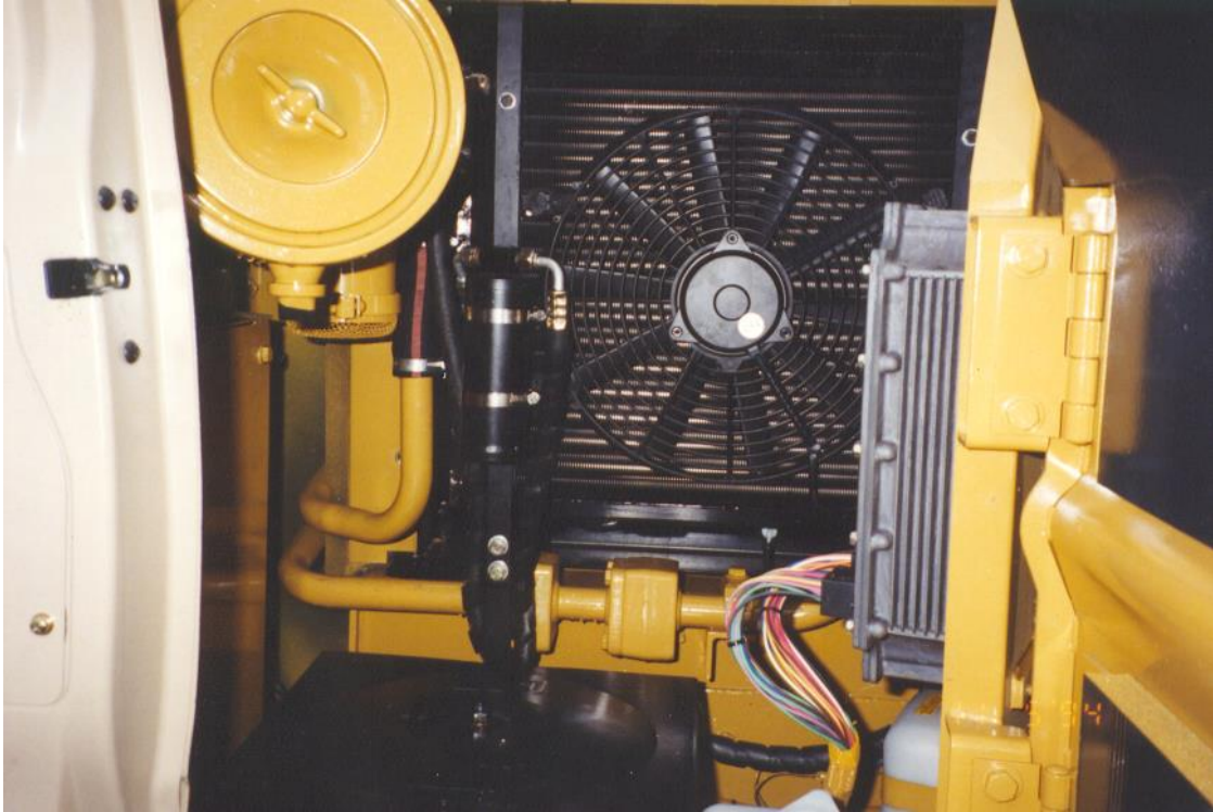
Condenser view. **NOTE** Fan no longer used.
